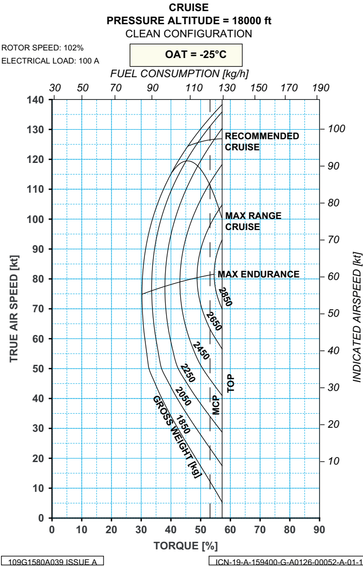
Figure 9-46. OAT = -25 °C - Altitude Pressure = 18000 ft
