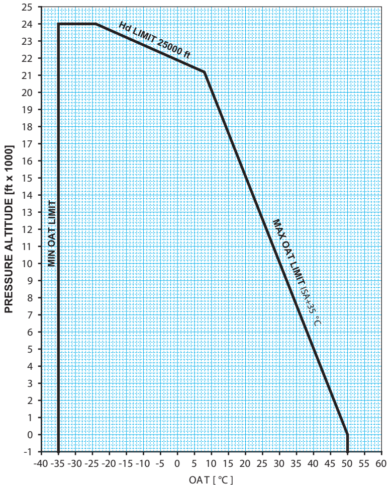
Figure 1-2. Pressure Altitude / OAT Envelope
