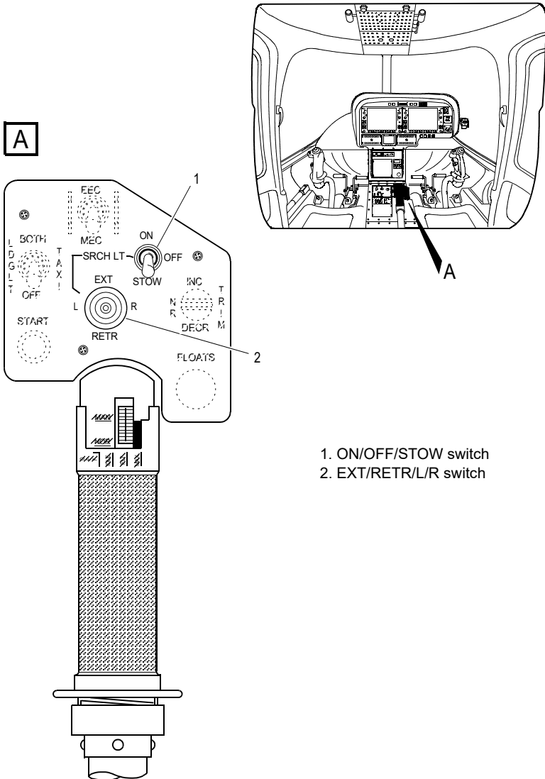
Figure 7-1. Searchlight Controls
