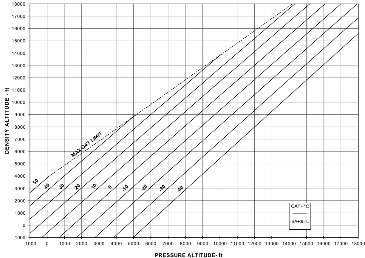
WEIGHT-ALTITUDE-TEMPERATURE DIAGRAM FOR LOW SPEED CONTROLLABILITY IGE-OGE
