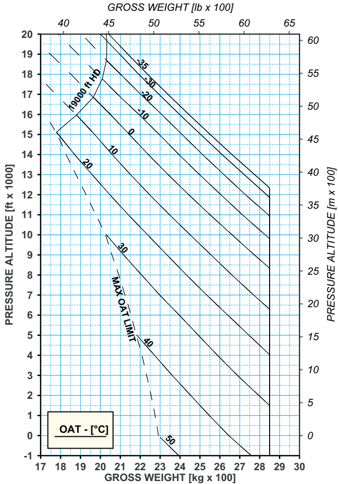
Figure 4-4. In Ground Effect (IGE) - Maximum Continuous Power (MCP) (Heater Off)
