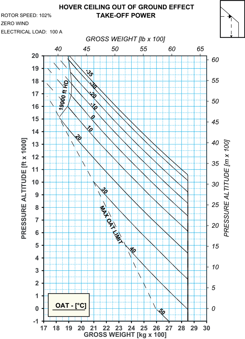
Figure 4-5. Out Ground Effect (OGE) - Take-Off Power (TOP) (Heater Off)
