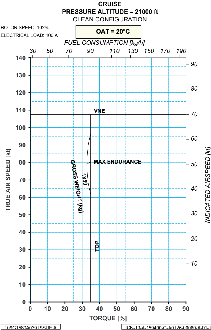
Figure 9-54. OAT = 20 °C - Altitude Pressure = 21000 ft
