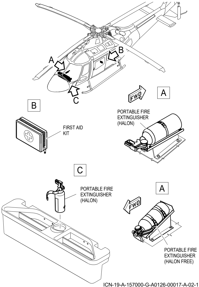
Figure 7-25. Emergency Equipment
