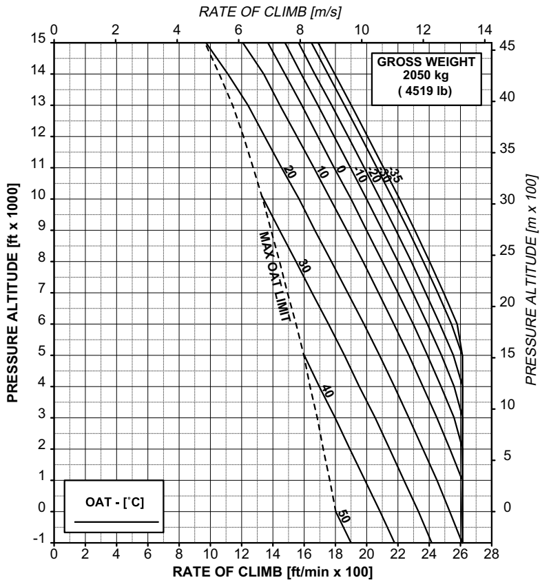
Figure 4-15. Take-Off Power (TOP) (Heater Off) - Gross Weight 2050 kg
