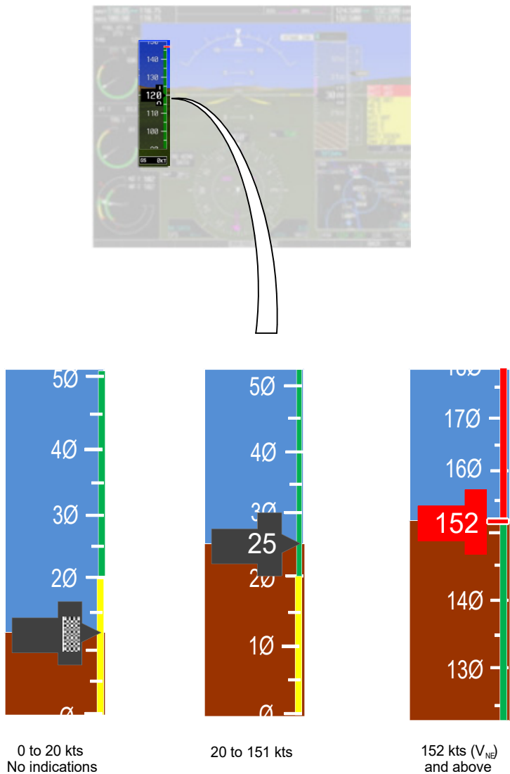
Figure 1-6. PFD Airspeed indicator
