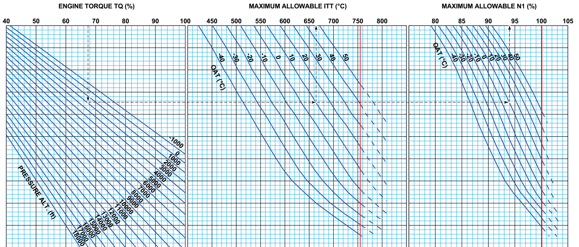
Figure 4-1. Power Assurance Check - Hover
