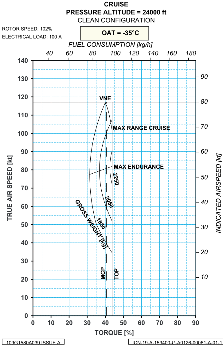
Figure 9-55. OAT = -35 °C - Altitude Pressure = 24000 ft
