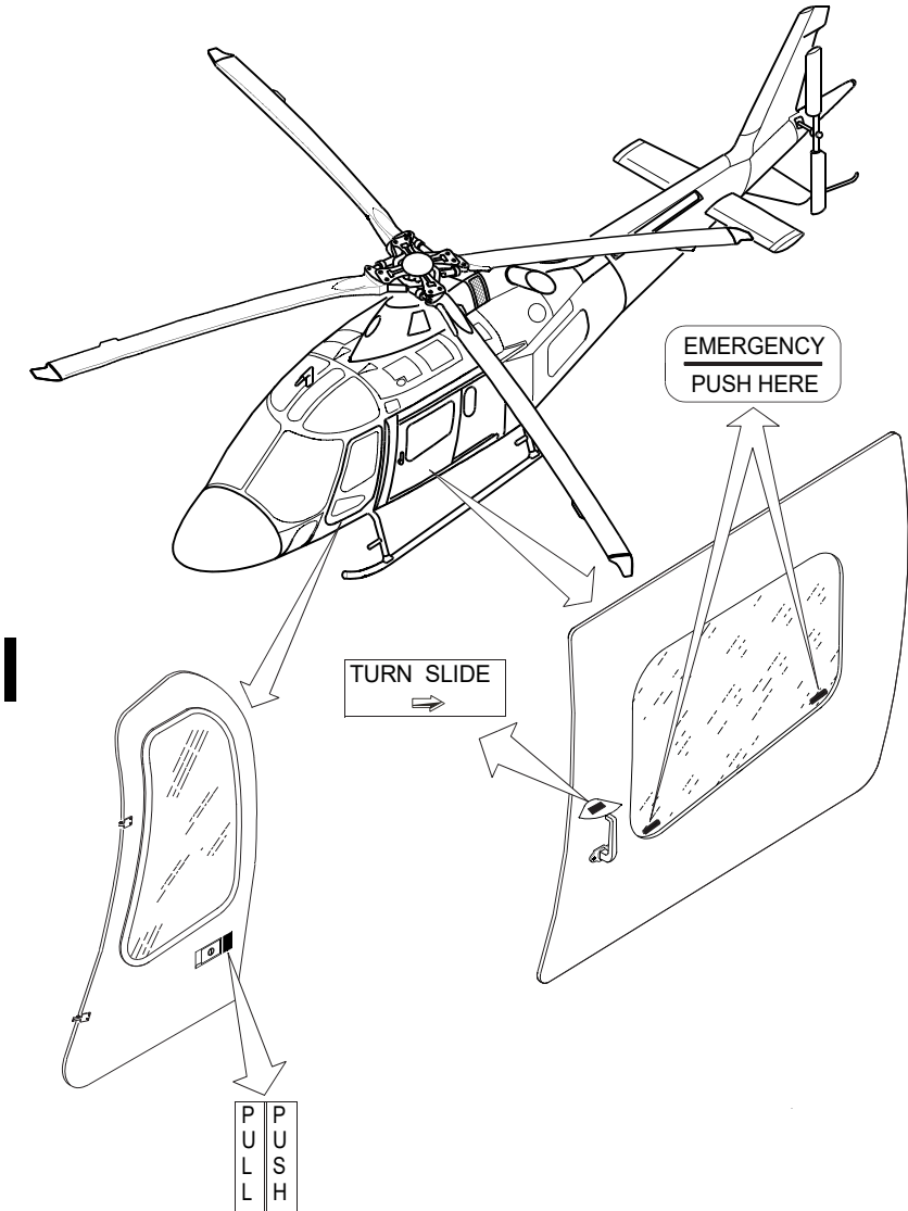
Figure 3-4. External Markings
