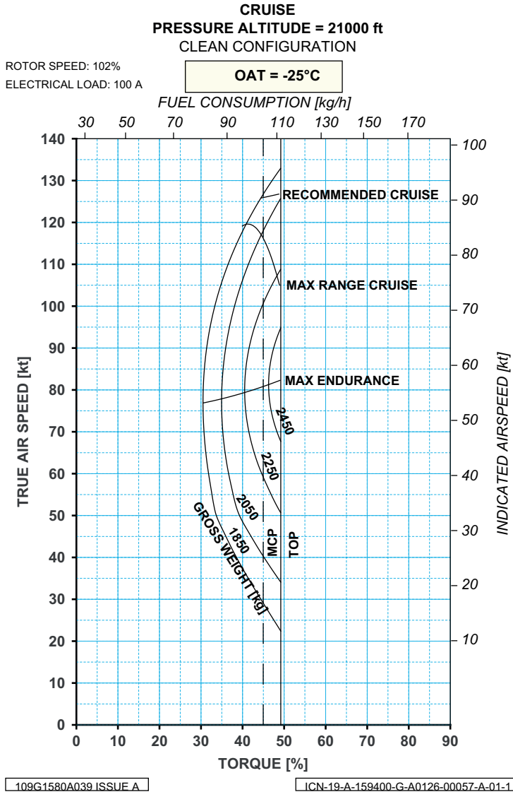
Figure 9-51. OAT = -25 °C - Altitude Pressure = 21000 ft
