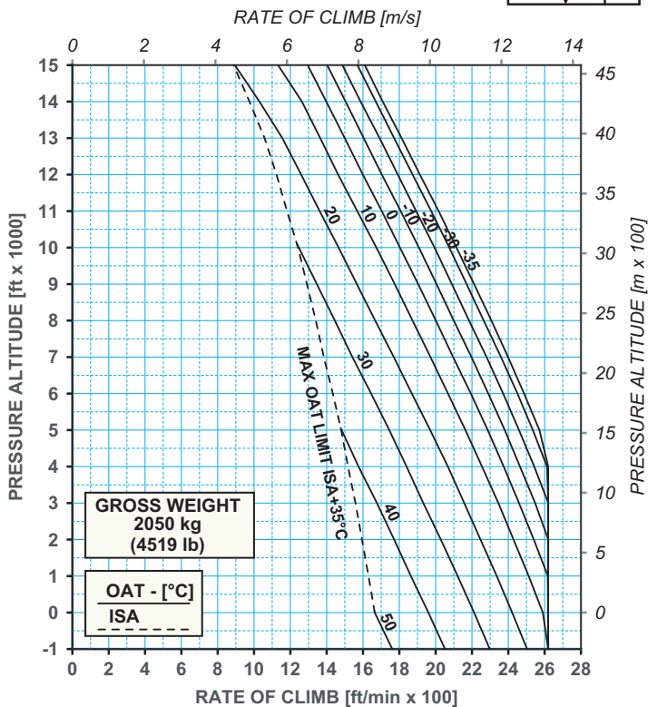
Figure 9-77. Rate Of Climb - Take-Off Power (TOP) - Gross Weight 2050 kg - IBF Clogged
