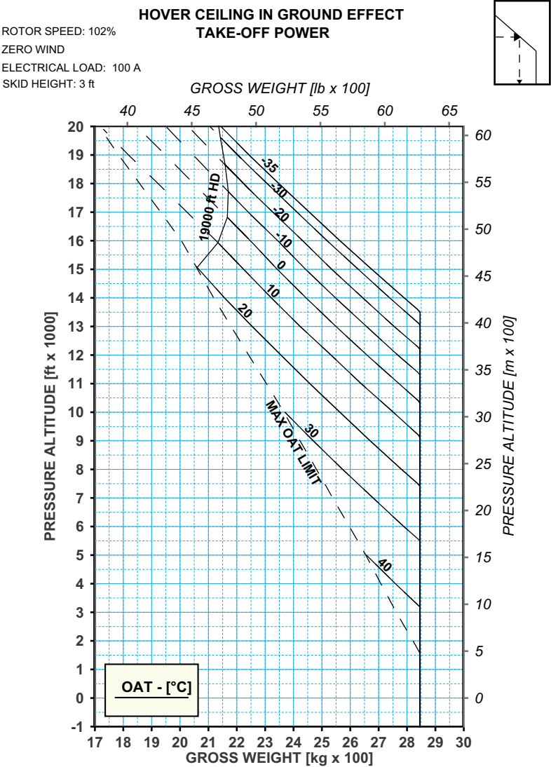
Figure 4-3. In Ground Effect (IGE) - Take-Off Power (TOP) (Heater Off)
