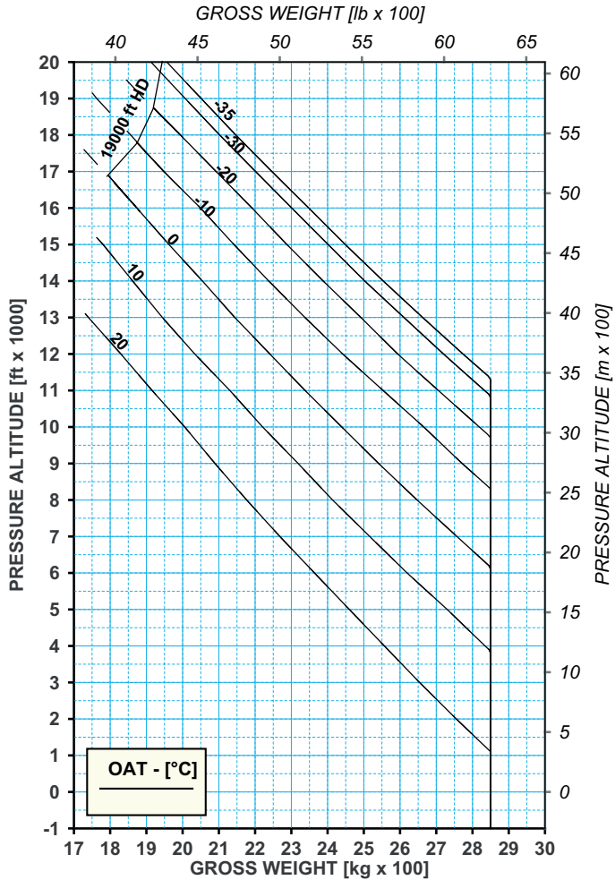
Figure 4-8. In Ground Effect (IGE) - Maximum Continuous Power (MCP) (Heater On)
