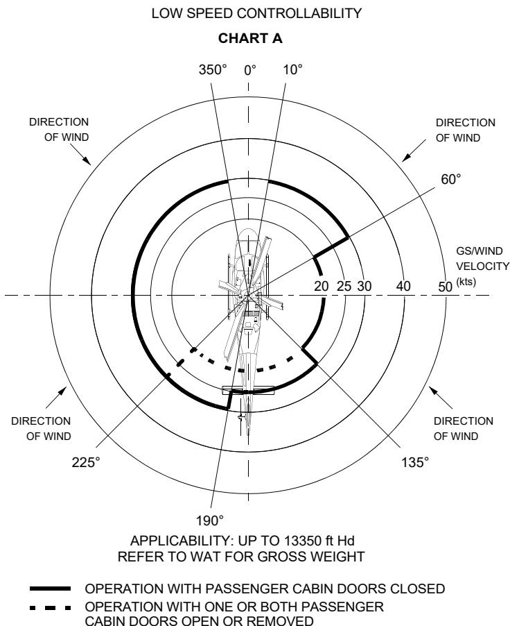
Figure 4-1. Wind/Ground Speed Azimuth Envelope (sheet 1 of 2).
