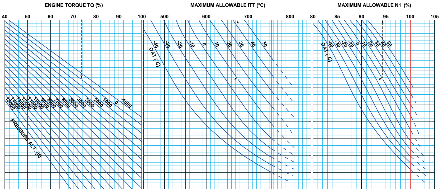
Figure 4-6. Power Assurance Check - In Flight (130 KIAS)
