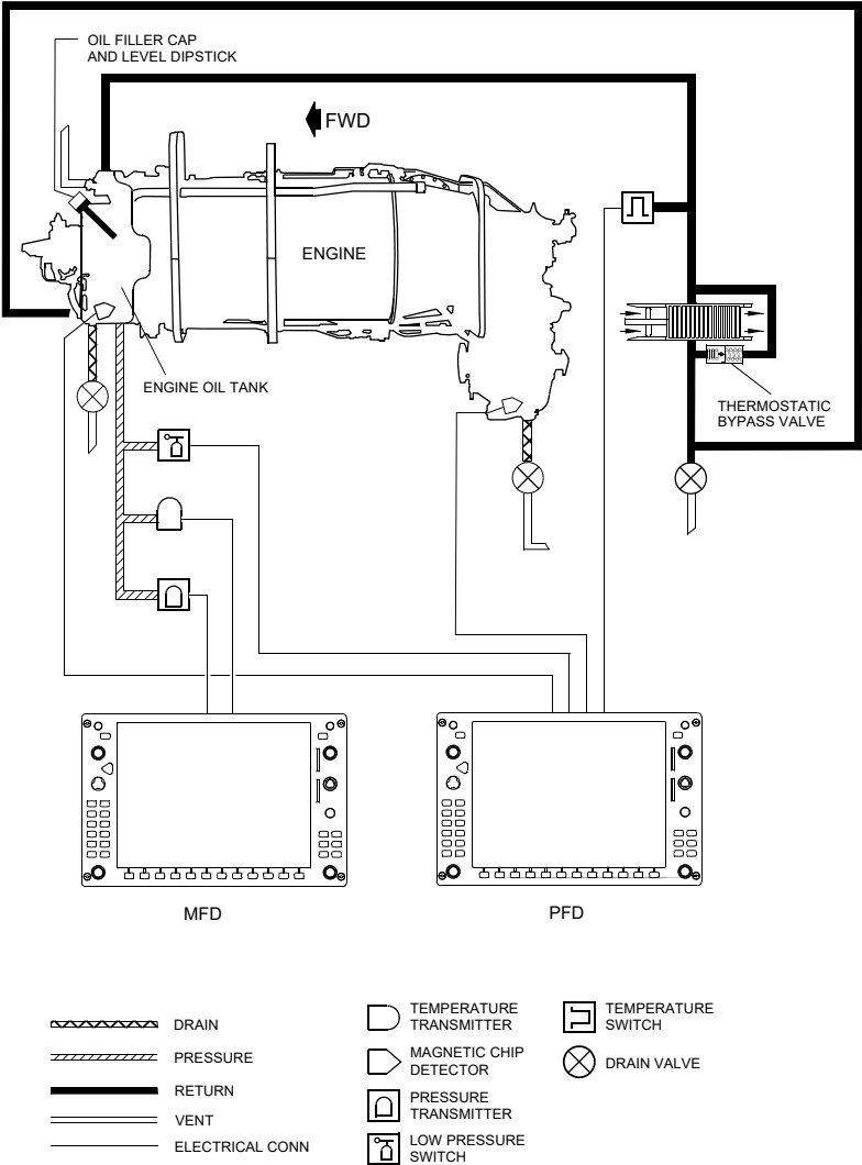
Figure 7-16. Engine Oil System Schematic
