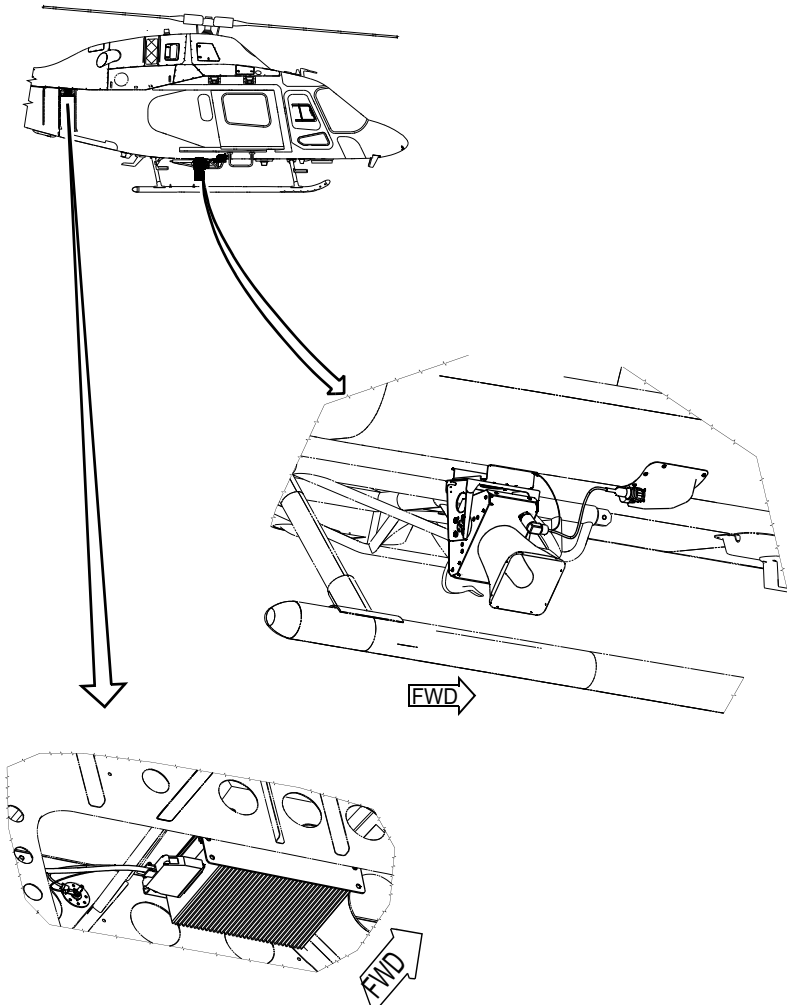
Figure 7-1. External Loudspeaker - Component Location
