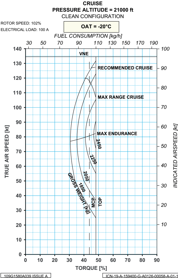
Figure 9-52. OAT = -20 °C - Altitude Pressure = 21000 ft
