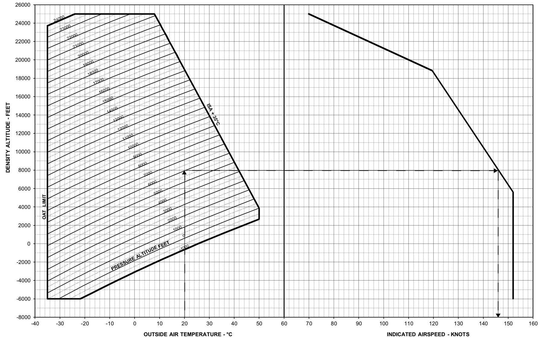
Figure 1-1. Airspeed Limitation - V NE (power on/off)
