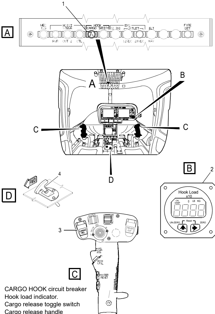
Figure 7-1. Cargo Hook Controls and Indicators
