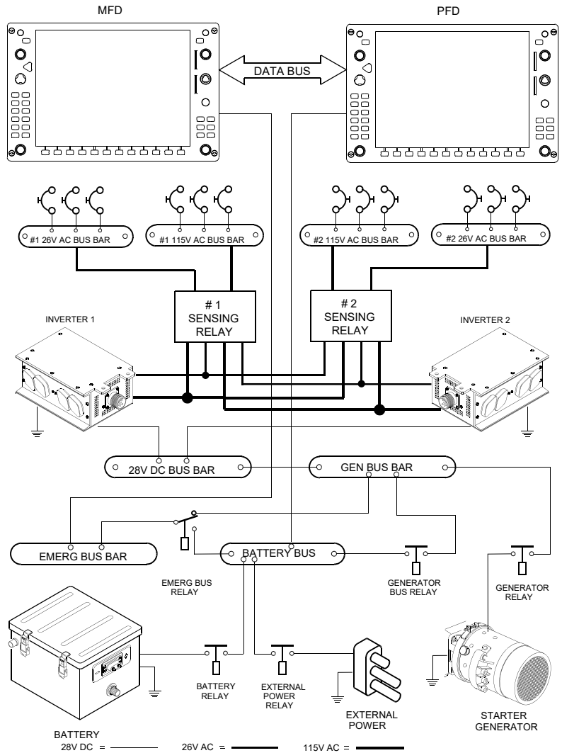
Figure 7-22. Electrical Power Schematic
