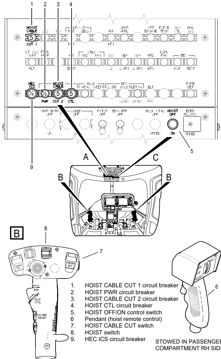
Figure 7-1. Hoist Controls
