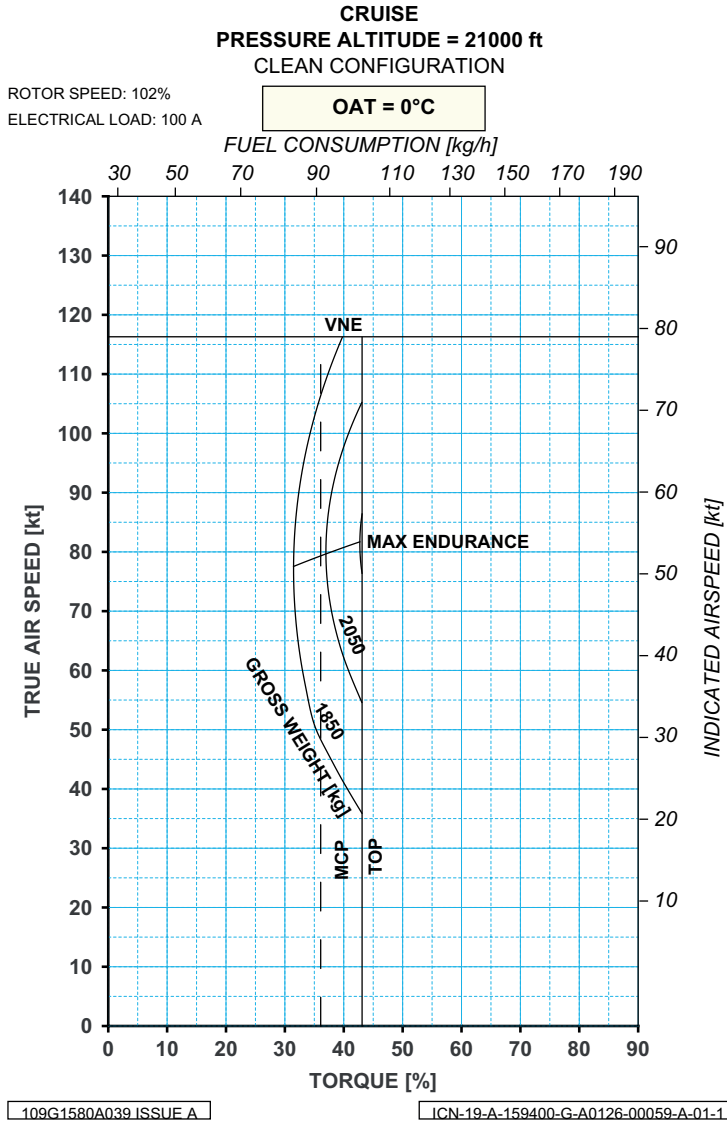
Figure 9-53. OAT = 0 °C - Altitude Pressure = 21000 ft
