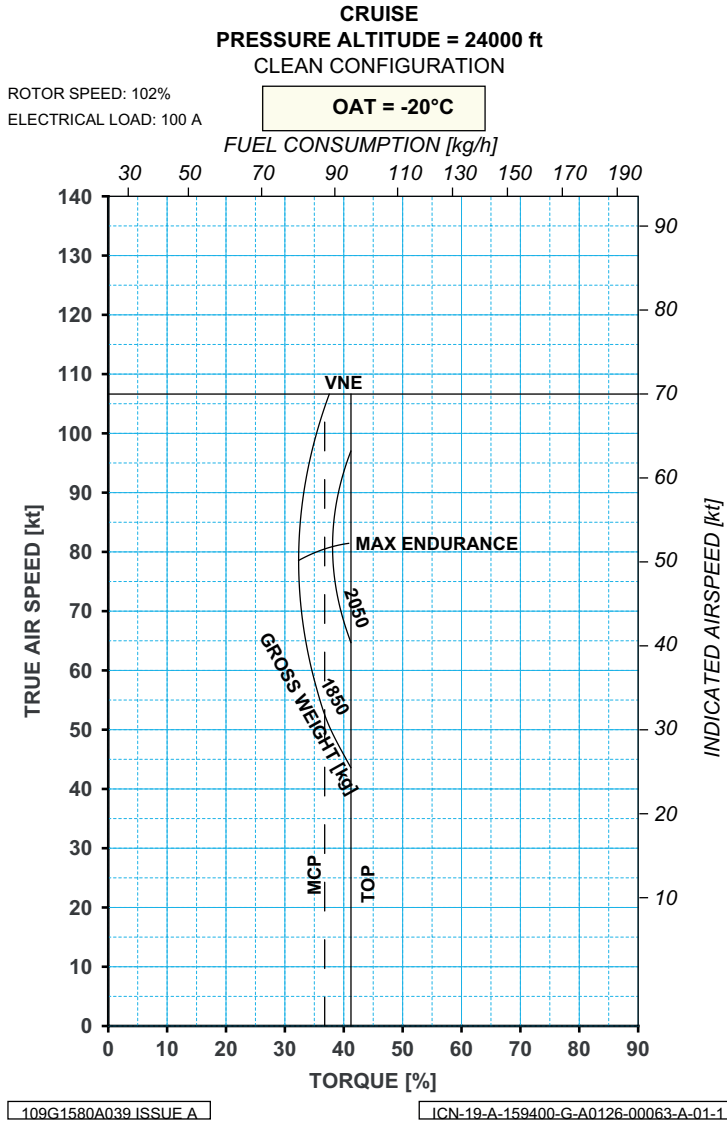
Figure 9-57. OAT = -20 °C - Altitude Pressure = 24000 ft
