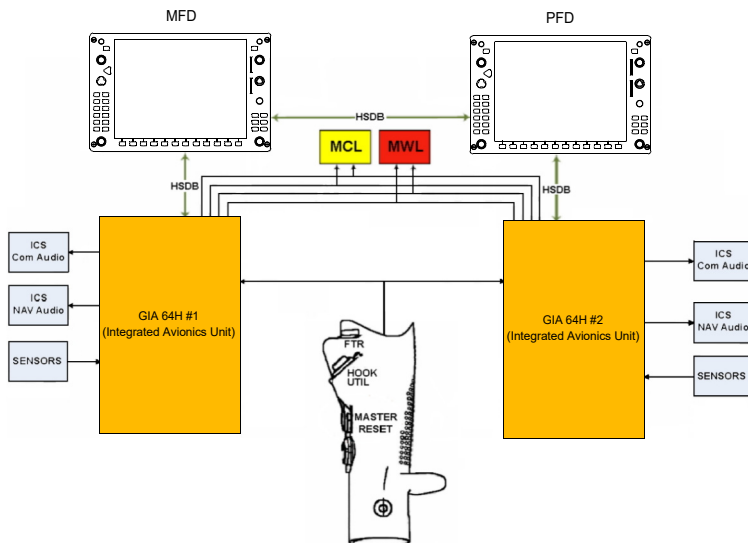
Figure 7-14I. Caution / Warning System Architecture
