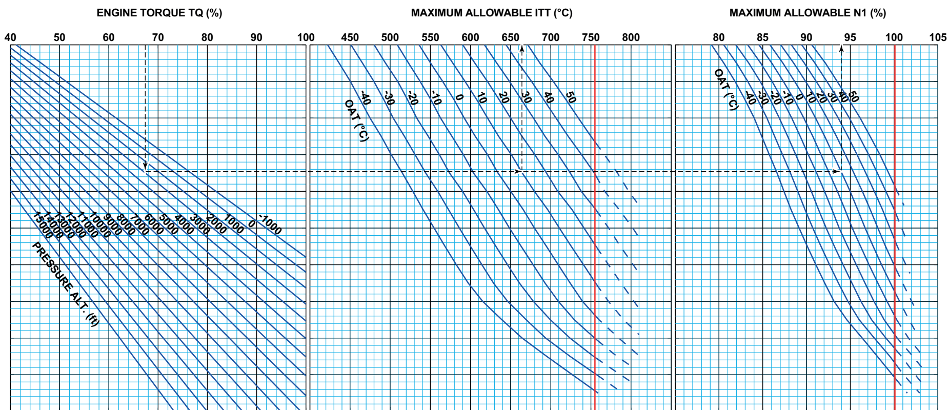
Figure 4-5. Power Assurance Check - Hover
