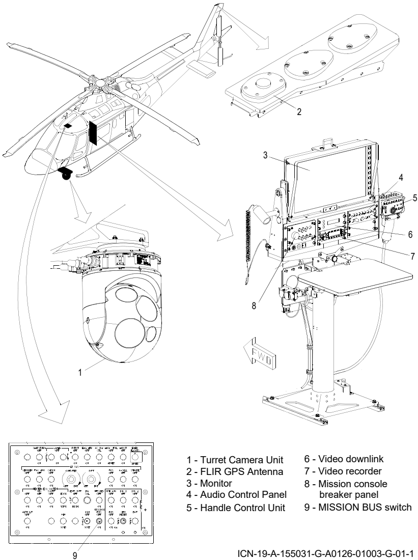
Figure 7-1. Flir MX-10 installation (G1000H NXi only) (sheet 2 of 2)
