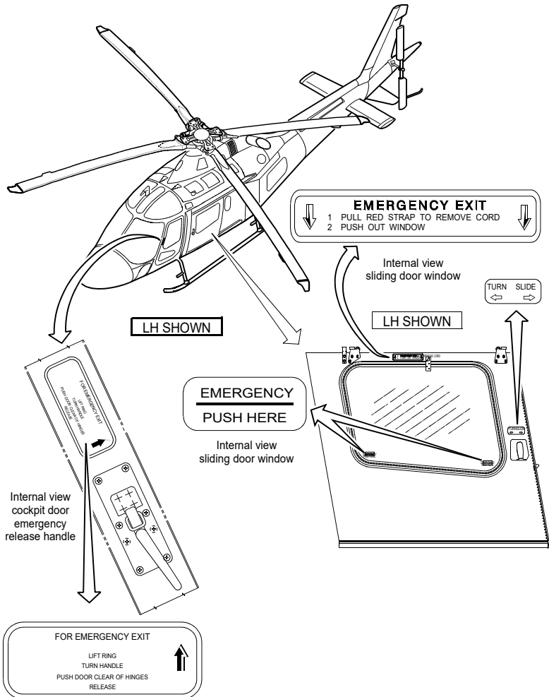
Figure 3-3. Internal Markings
