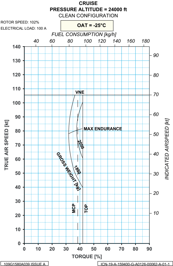
Figure 9-56. OAT = -25 °C - Altitude Pressure = 24000 ft
