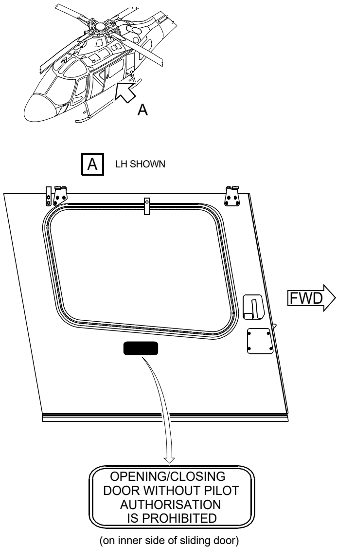
Figure 1-19. Cabin Placards
