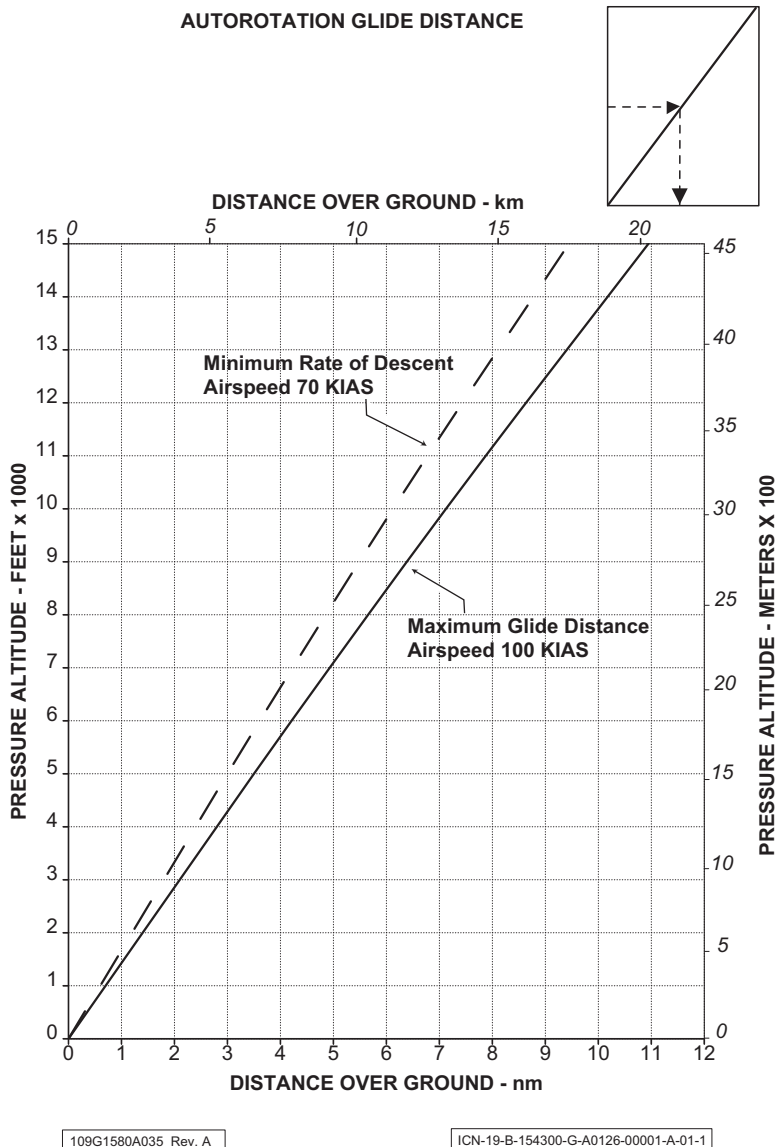
Figure 4-25. Autorotation Glide Distance
