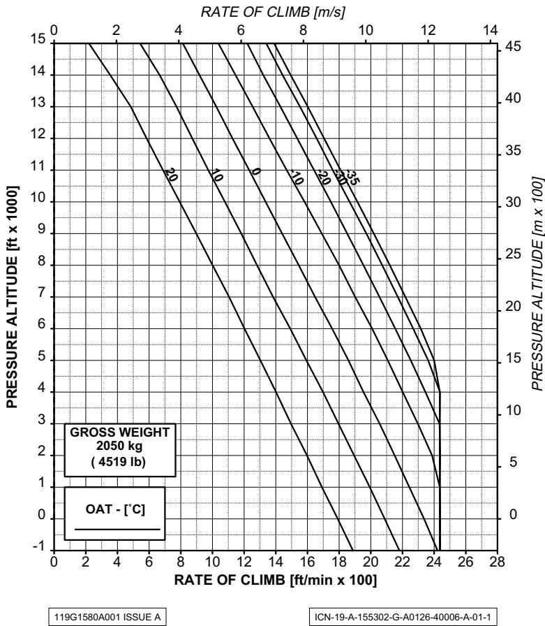
Figure 4-10. Maximum Continuous Power (MCP) (Heater ON) - Gross Weight 2050 kg
