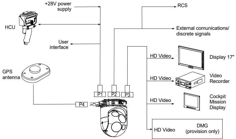
Figure 7-2. Mission System Configuration (G1000H only) (sheet 1 of 2)
