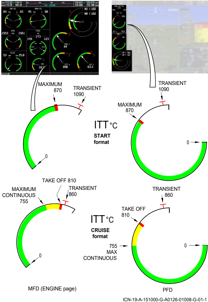
Figure 1-11. Inter Turbine Temperature (ITT)
