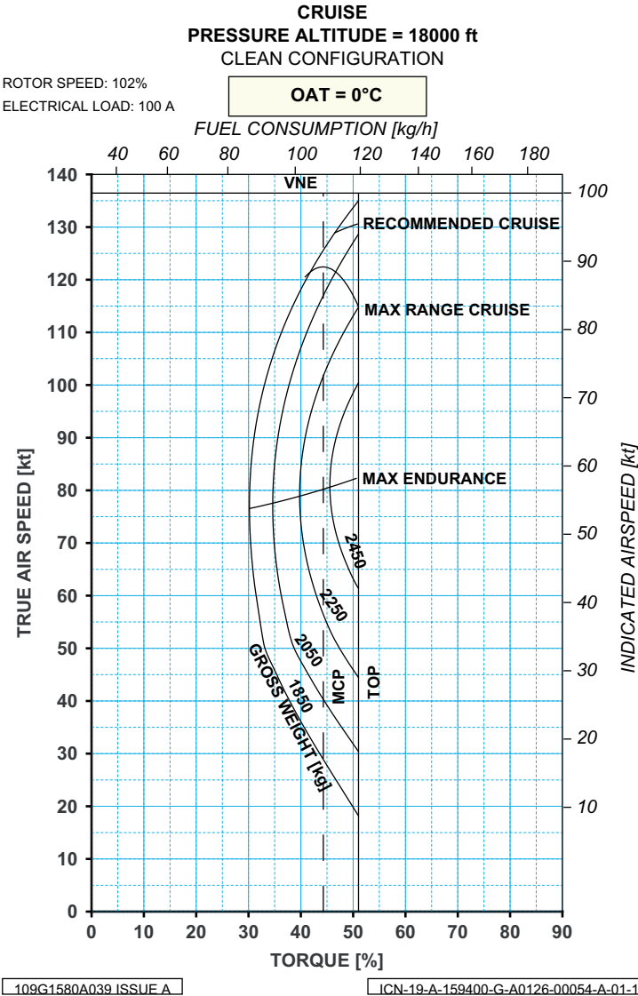
Figure 9-48. OAT = 0 °C - Altitude Pressure = 18000 ft
