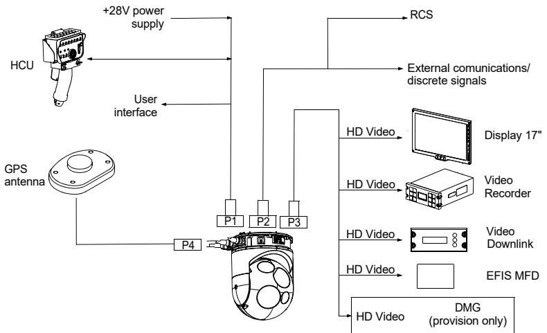
Figure 7-2. Mission System Configuration (G1000H NXi only) (sheet 2 of 2)
