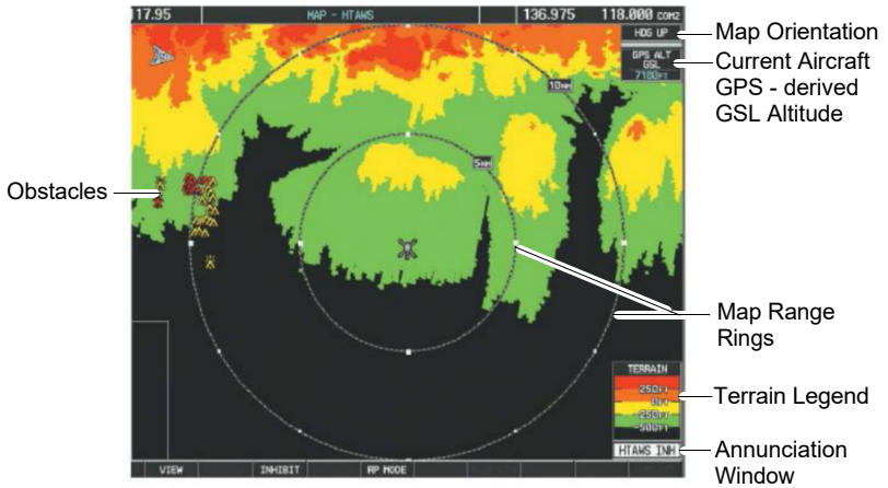
Figure 7-14F. HTAWS Page (360 View) (for reference only)
