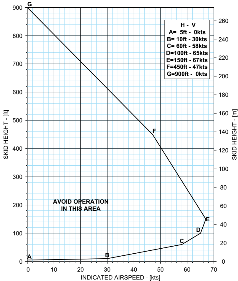
Figure 4-14. Height - Velocity Diagram - Chart B
