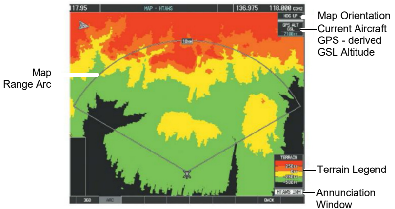
Figure 7-14G. HTAWS Page (Arc View) (for reference only)
