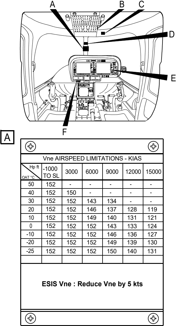
Figure 1-18. Cockpit Placards (sheet 1 of 2)
