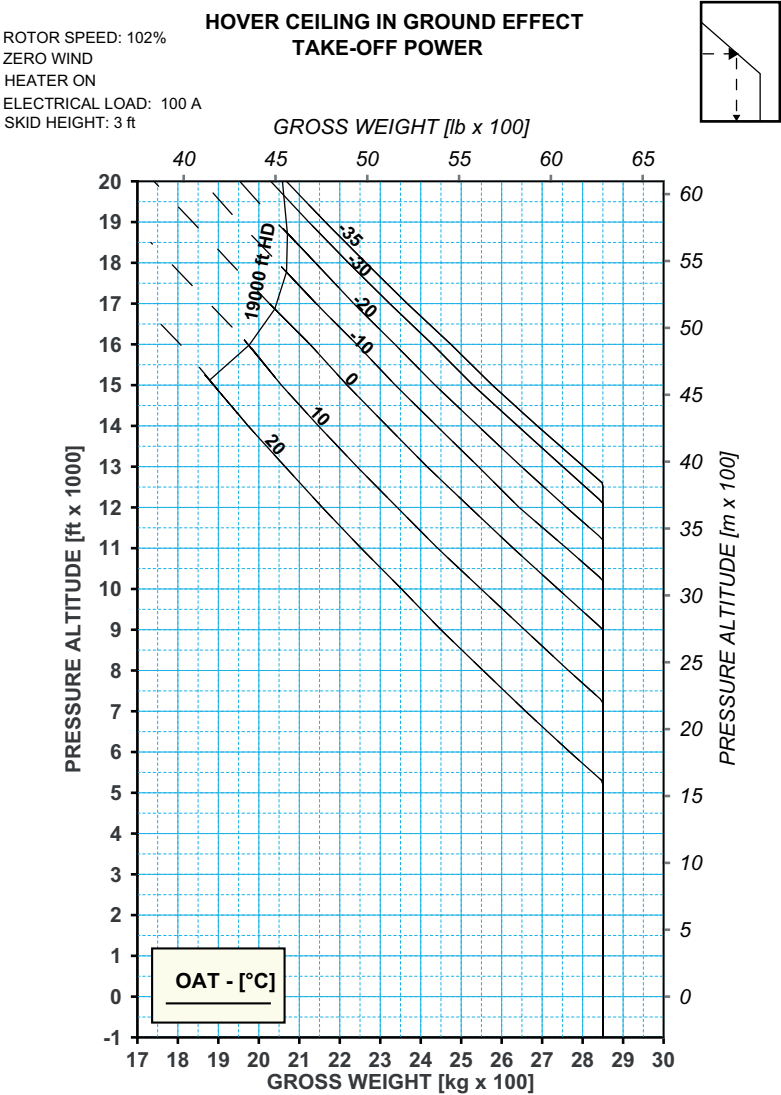
Figure 4-7. In Ground Effect (IGE) - Take-Off Power (TOP) (Heater On)
