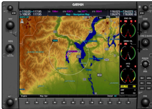
Figure 7-14C. Representative G1000H NXi Multi-Function Display (MFD) (for reference only)
