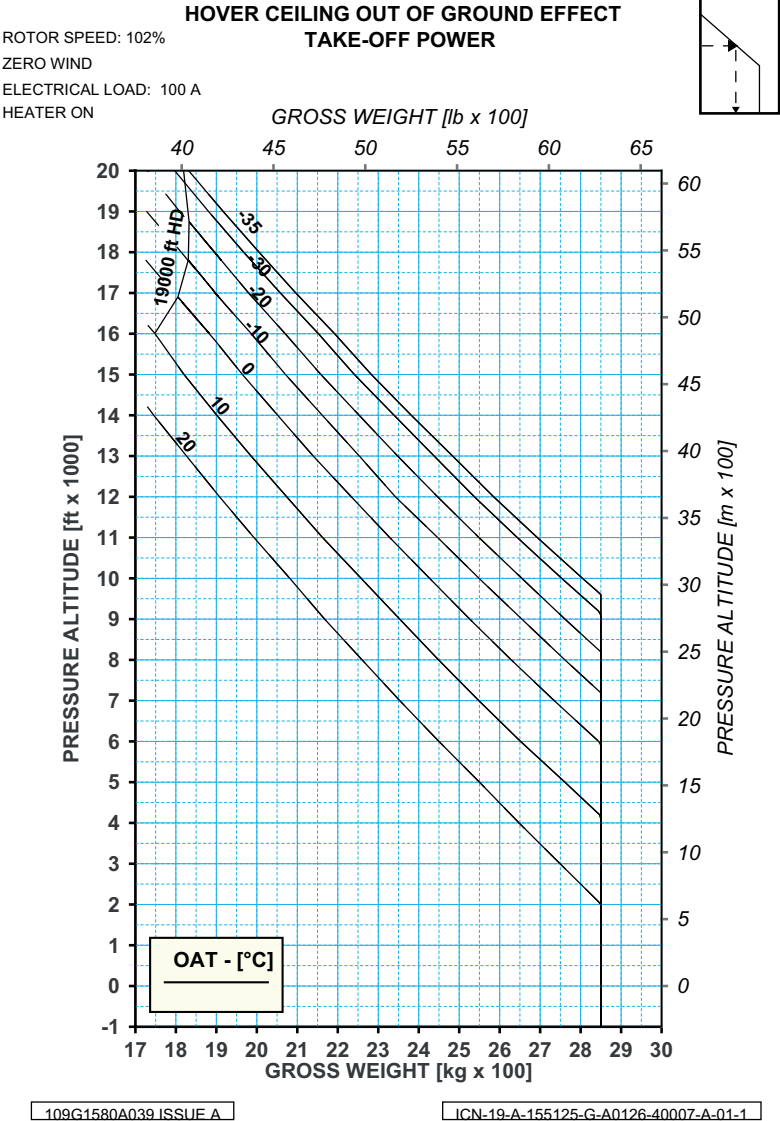
Figure 4-9. Out Ground Effect (OGE) - Take-Off Power (TOP) (Heater On)
