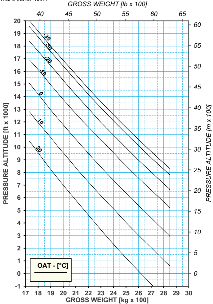
Figure 4-10. Out Ground Effect (OGE) - Maximum Continuous Power (MCP) (Heater On)
