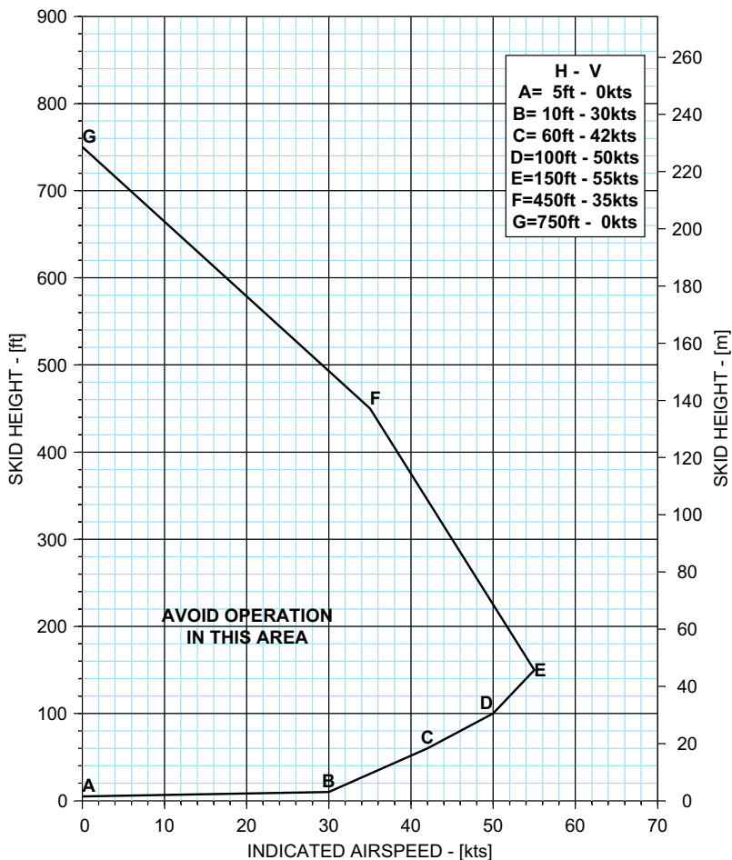
Figure 4-13. Height - Velocity Diagram - Chart A
