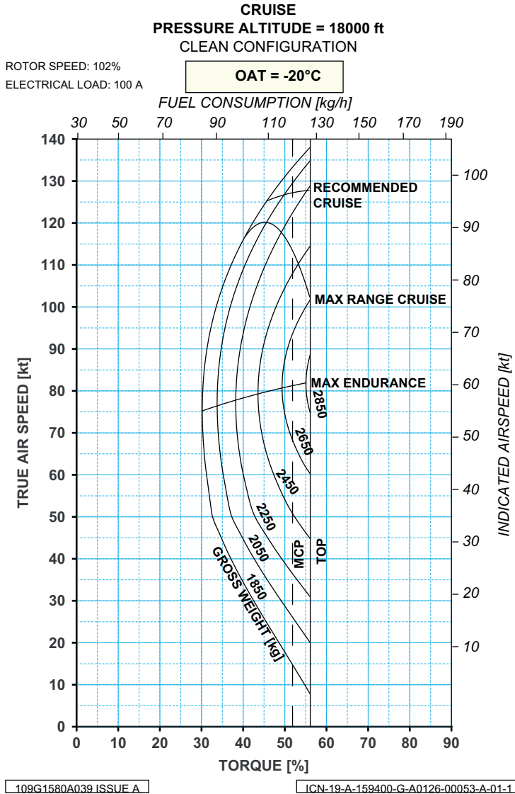
Figure 9-47. OAT = -20 °C - Altitude Pressure = 18000 ft
