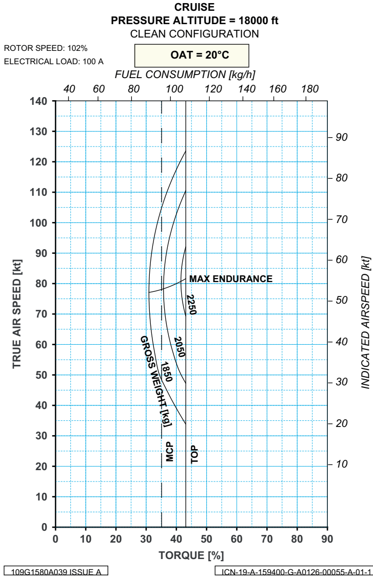
Figure 9-49. OAT = 20 °C - Altitude Pressure = 18000 ft
