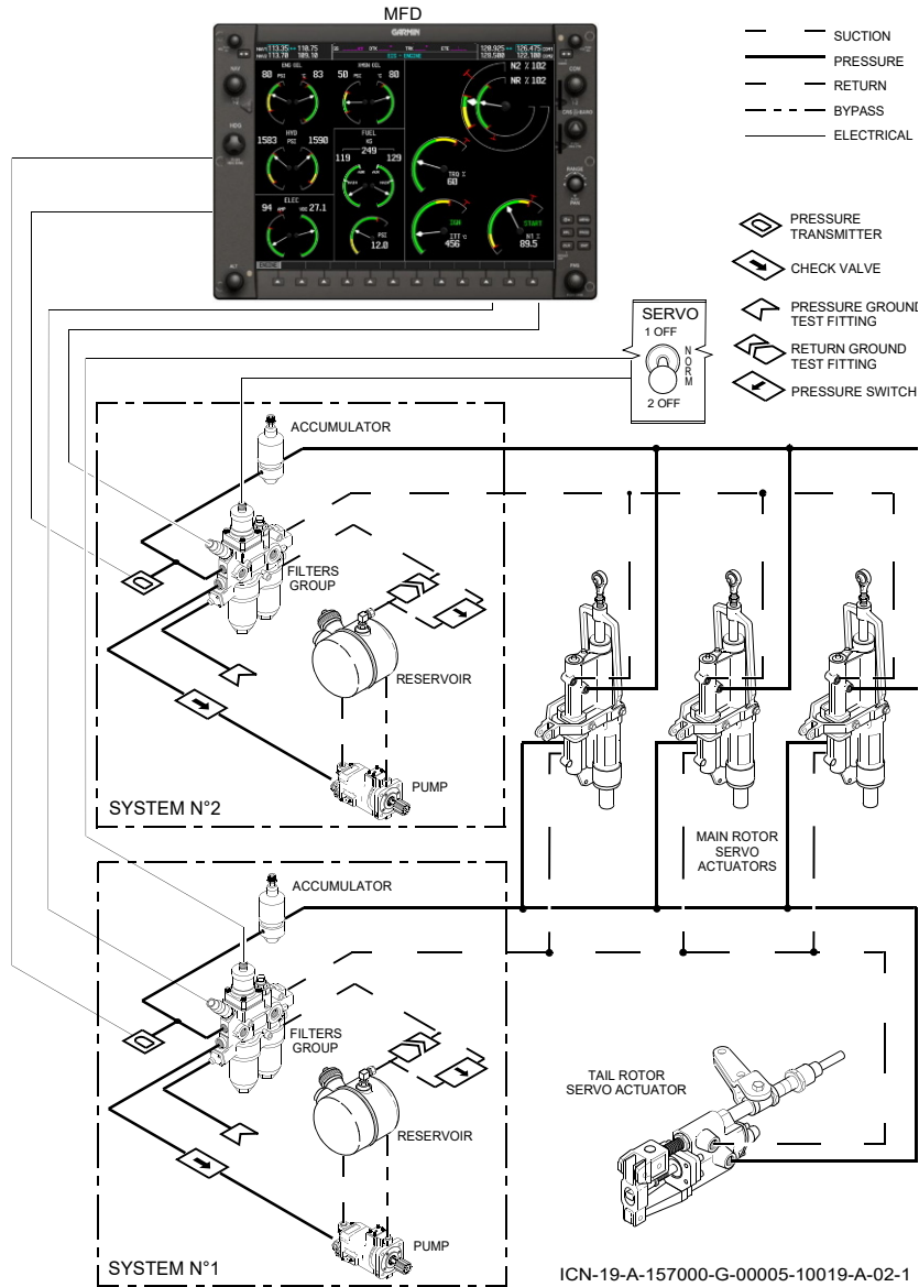
Figure 7-21. Hydraulic Power Schematic
