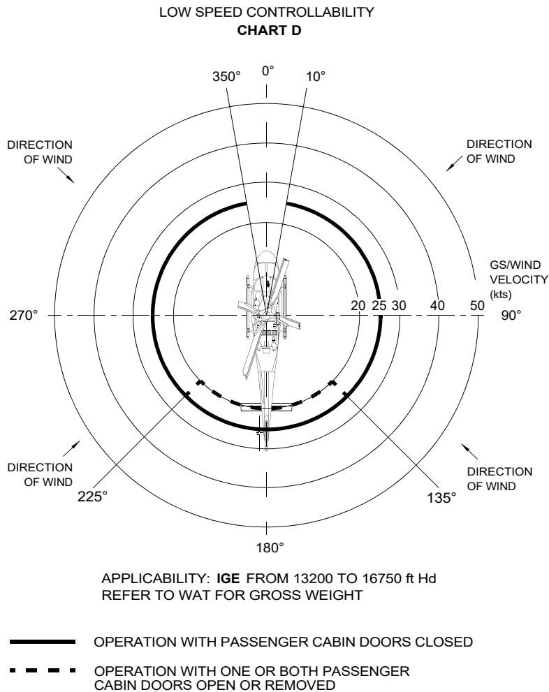
Figure 4-2. Wind/Ground Speed Azimuth Envelope (sheet 1 of 2)
