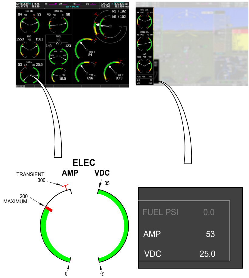
MFD (ENGINE and MAP pages)
