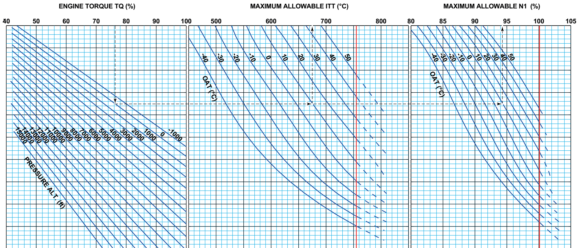
Figure 4-7. Power Assurance Check - In Flight (100 KIAS)
