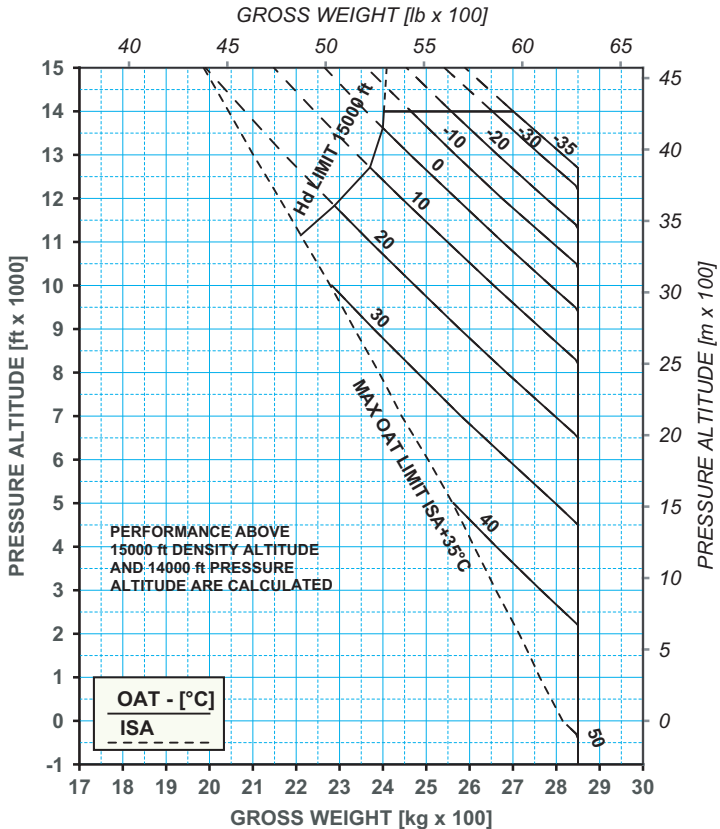
Figure 9-59. Hover Ceiling In Ground Effect (IGE) - Take-Off Power (TOP) - IBF Clogged
