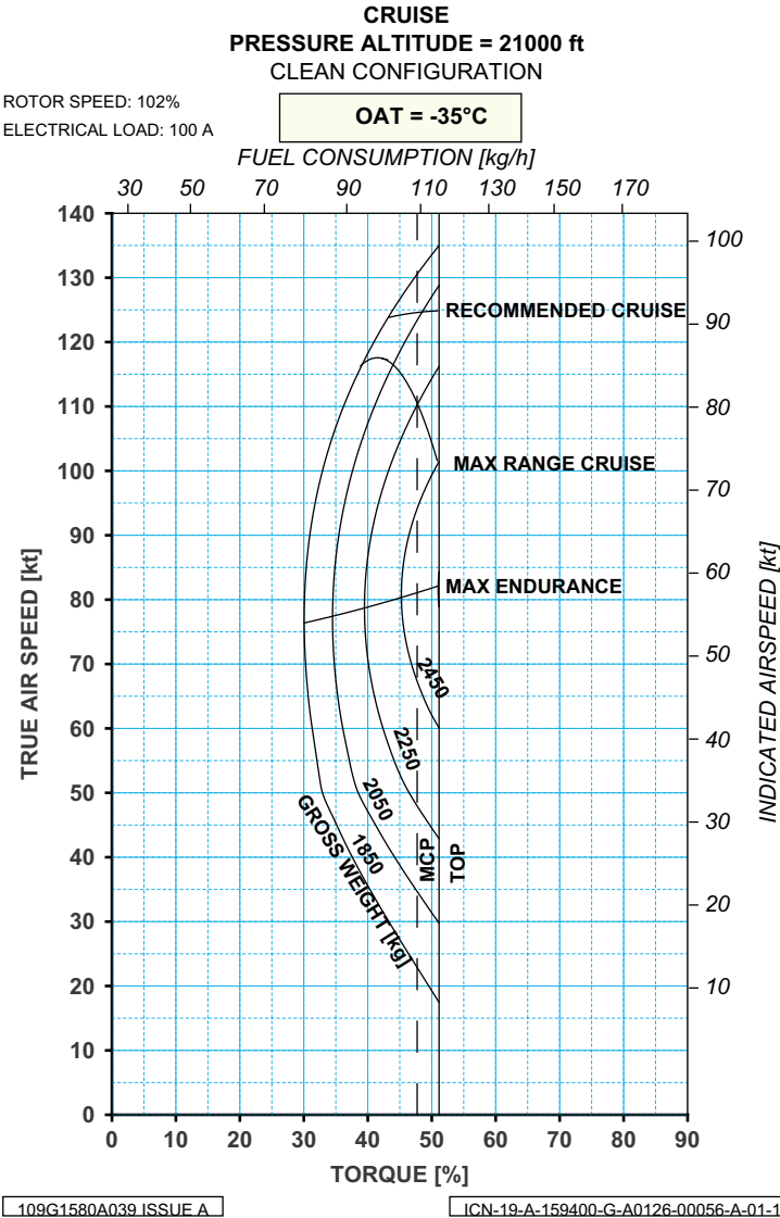
Figure 9-50. OAT = -35 °C - Altitude Pressure = 21000 ft
