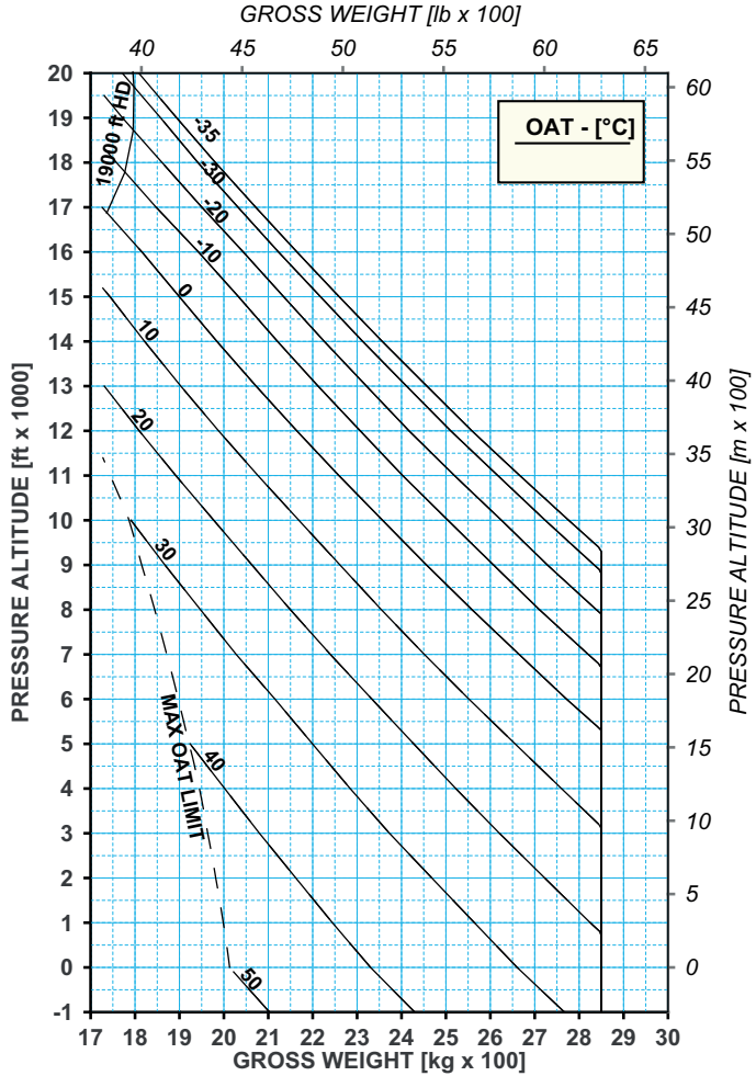
Figure 4-6. Out Ground Effect (OGE) - Maximum Continuous Power (MCP) (Heater Off)
