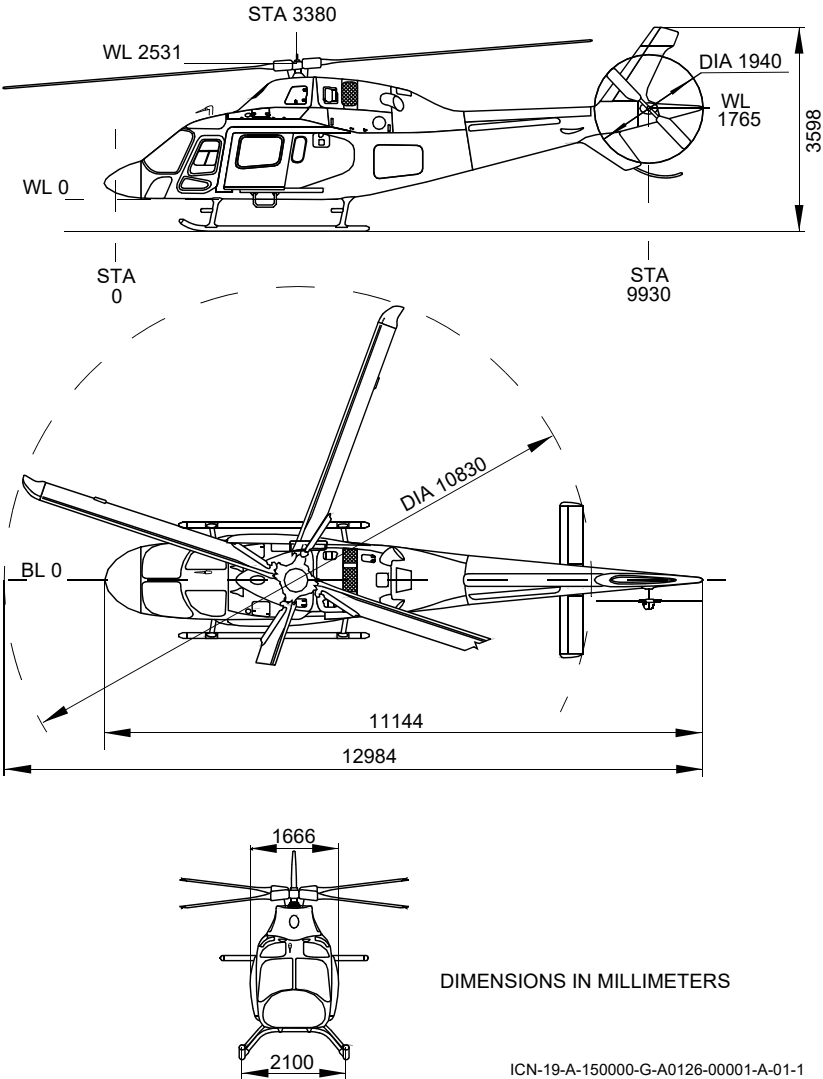
Figure 1. Helicopter — Three views
